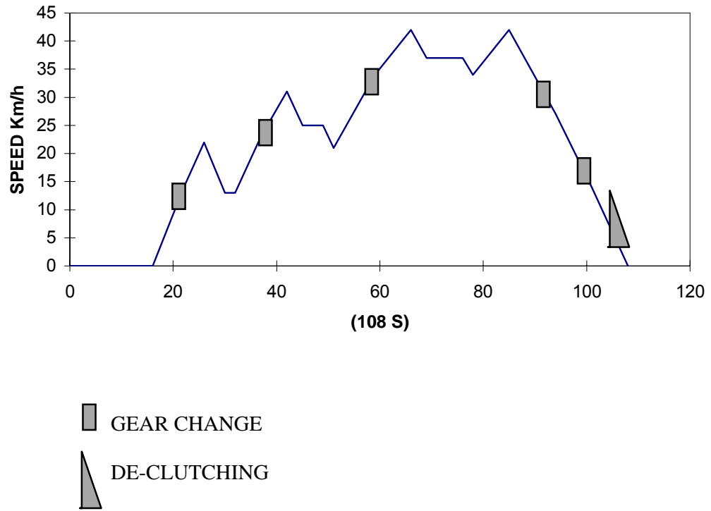
Fig 1 : OPERATING CYCLE WITH RECOMMENDED GEAR POSITION (Pl. ref. para 2.3.1.1.5)
