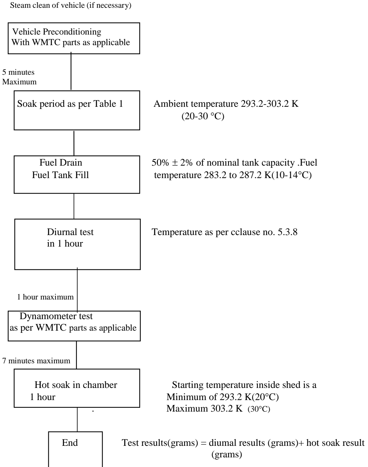
FIGURE 1. EVAPORATIVE EMISSION DETERMINATION SHED TEST
